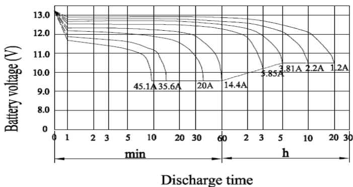
Discharge characteristic (25°C)
